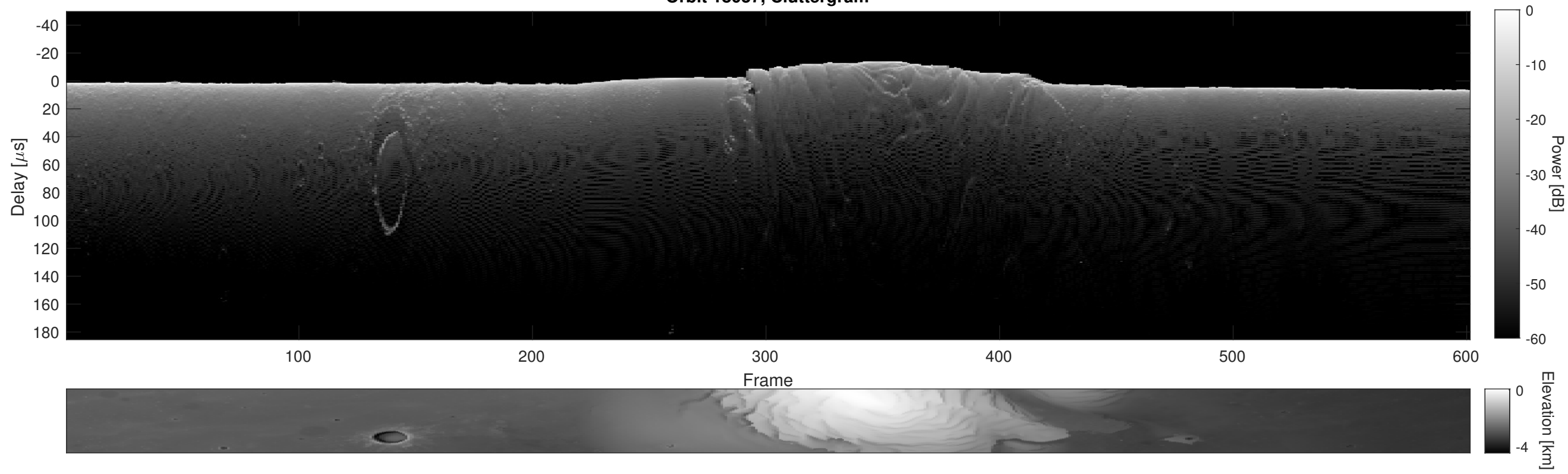
Orbit 18037, Cluttergram
