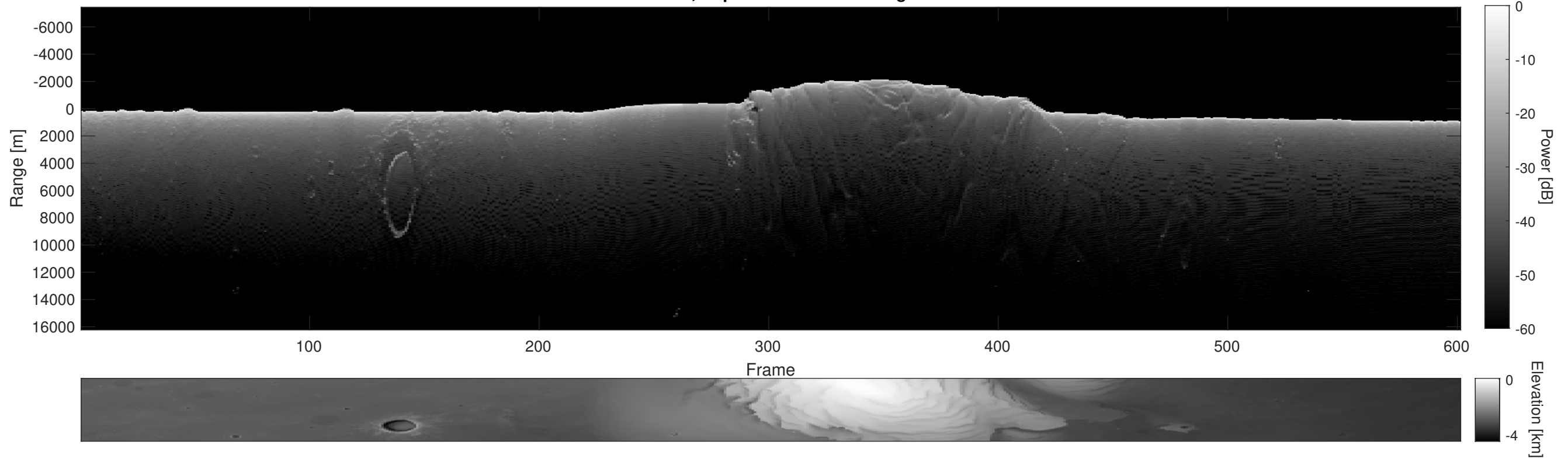
Orbit 18037, Depth-Corrected Cluttergram
