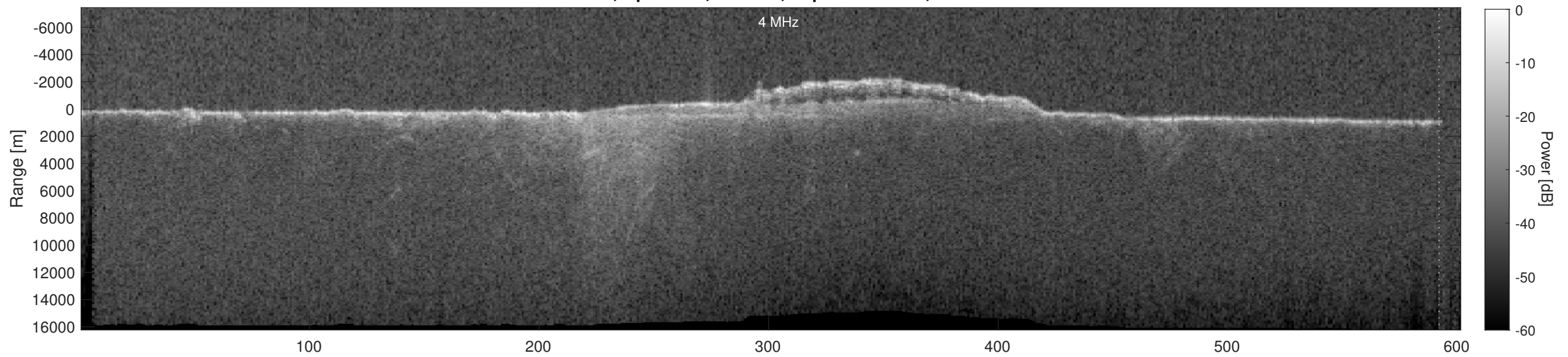
Orbit 18037, Depth-Corrected Cluttergram
