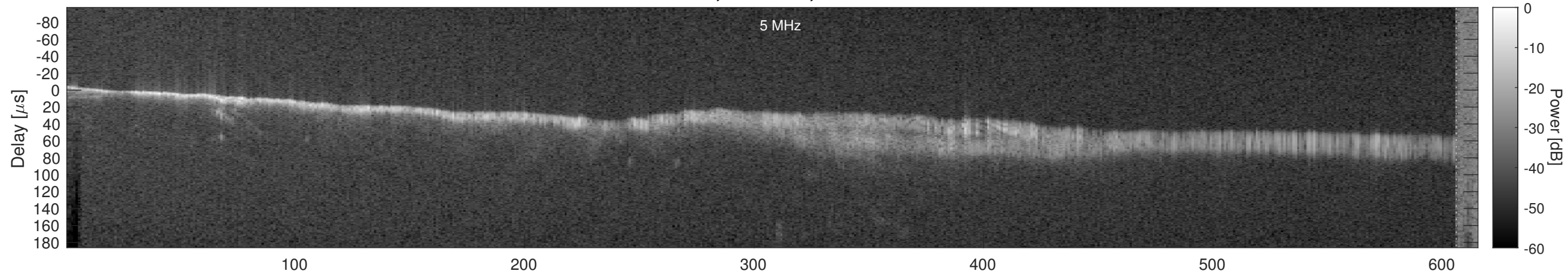
Orbit 18043, Window, Channel 1, Chapman
