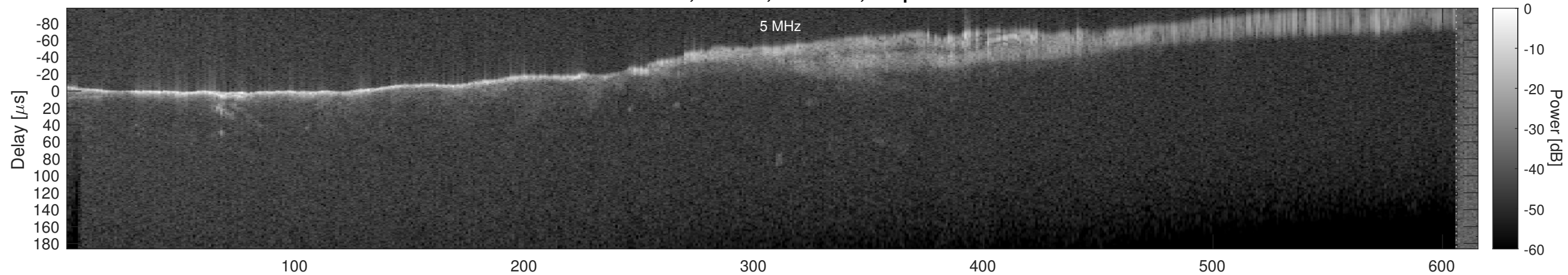
Orbit 18043, Window, Channel 1, Optimized
