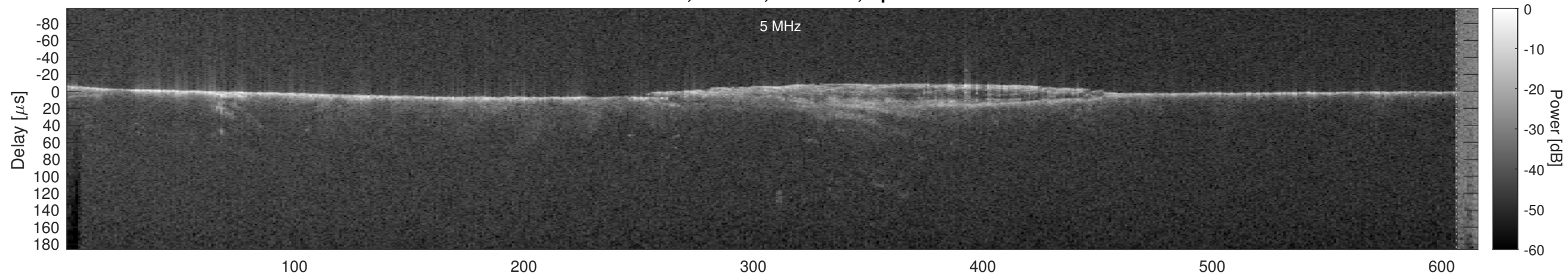
Orbit 18043, Cluttergram
