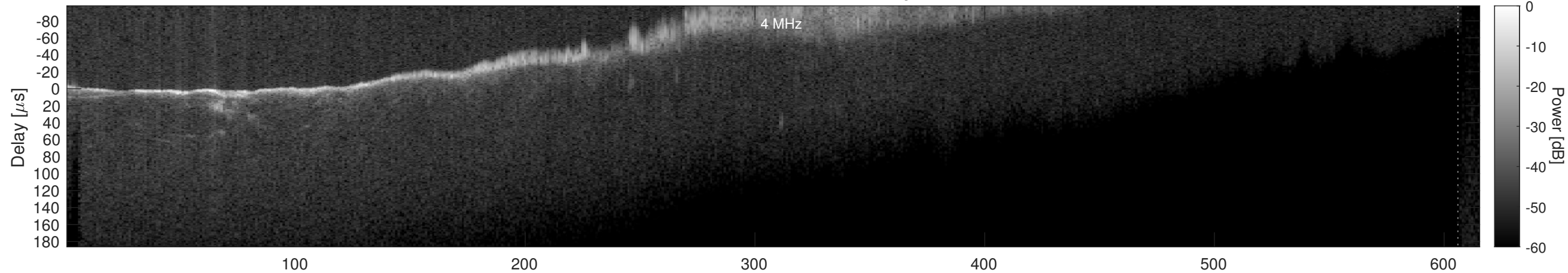
Orbit 18043, Window, Channel 2, Optimized
