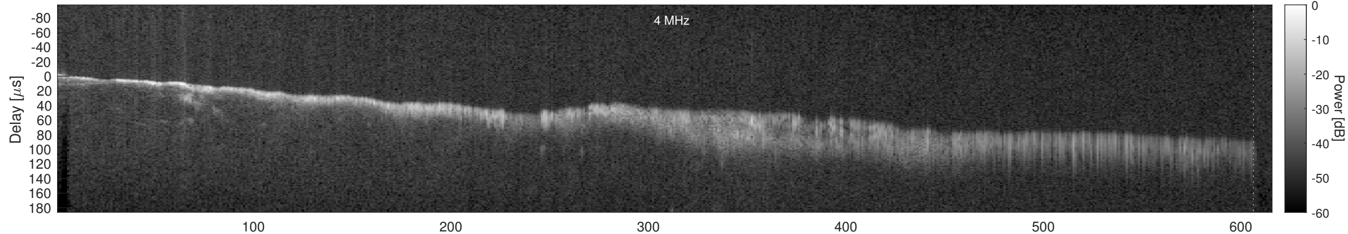
Orbit 18043, Window, Channel 2, Chapman
