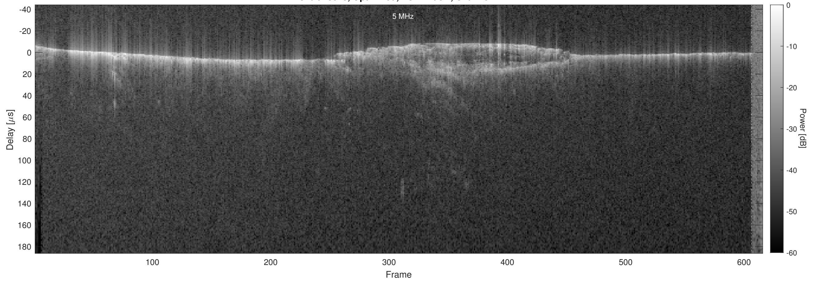
Orbit 18043, Optimized, No Window, Channel 2
