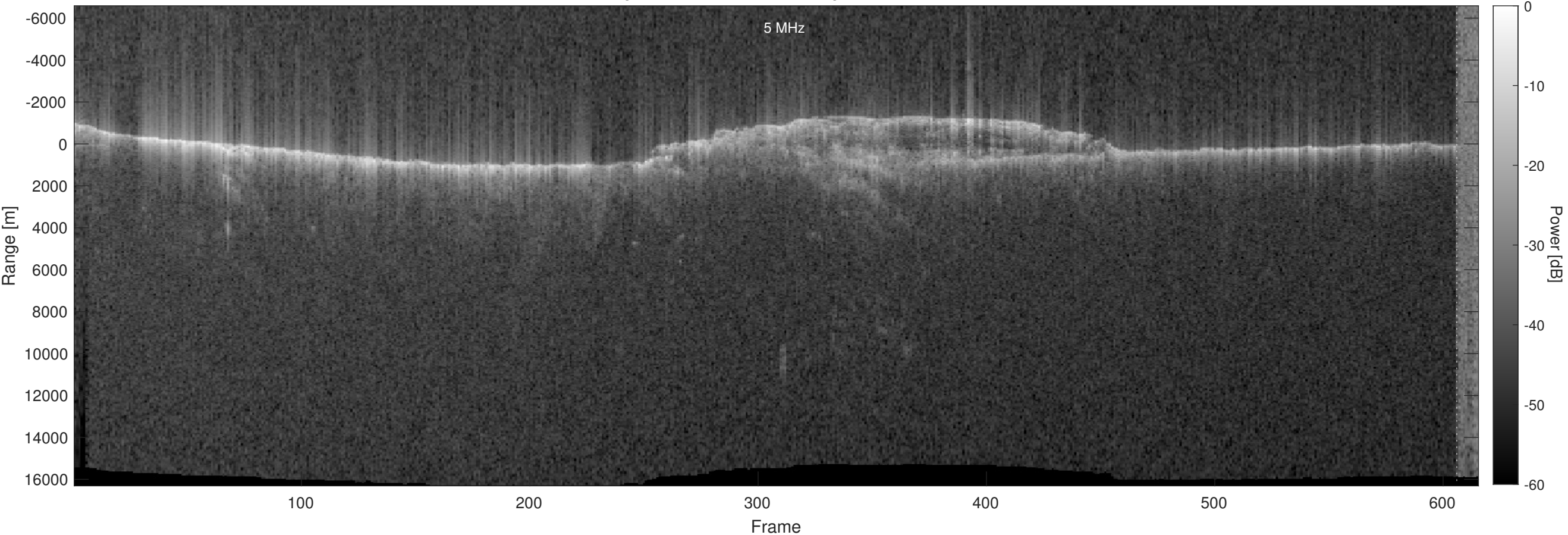
Orbit 18043, Optimized, No Window, Depth-Corrected, Channel 2
