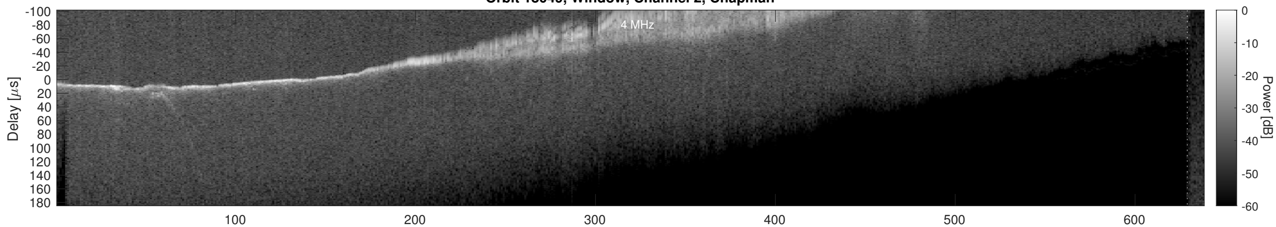
Orbit 18049, Window, Channel 2, Optimized
