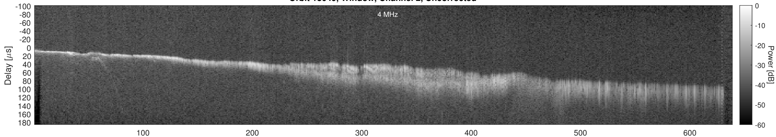
Orbit 18049, Window, Channel 2, Chapman
