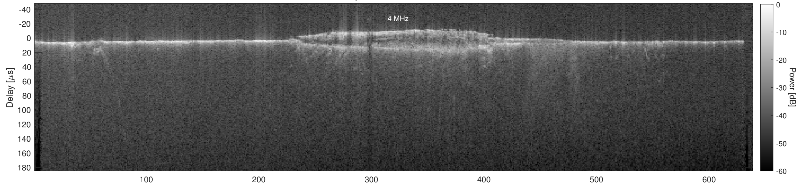
Orbit 18049, Cluttergram
