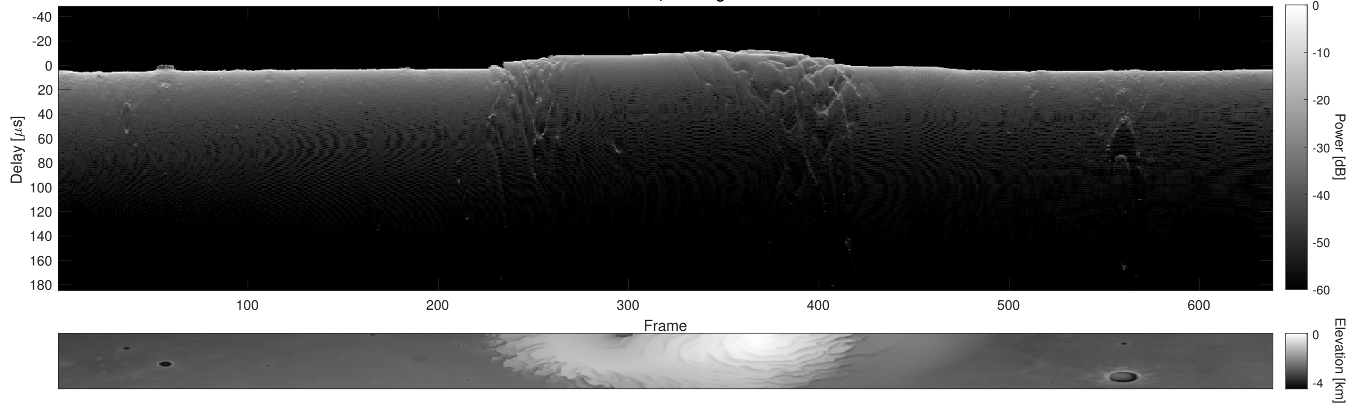
Orbit 18049, Cluttergram
