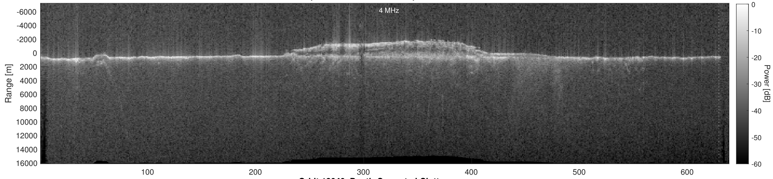
Orbit 18049, Depth-Corrected Cluttergram
