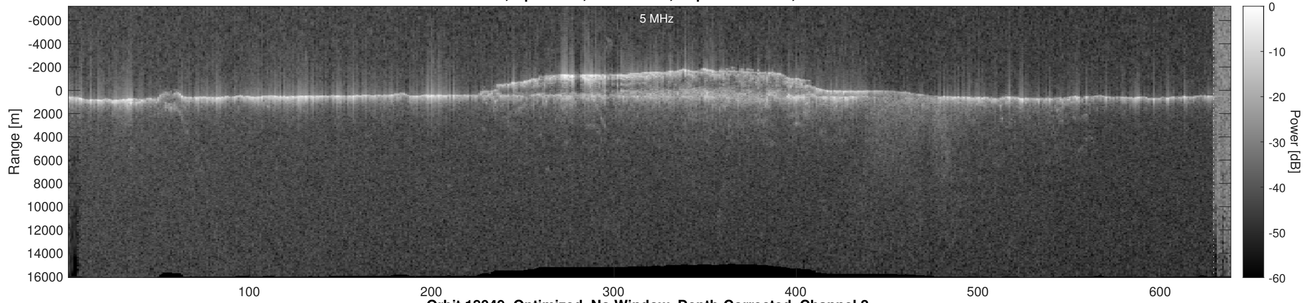
Orbit 18049, Optimized, No Window, Depth-Corrected, Channel 2
