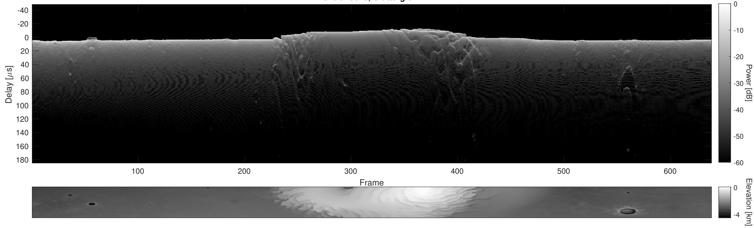
Orbit 18049, Cluttergram
