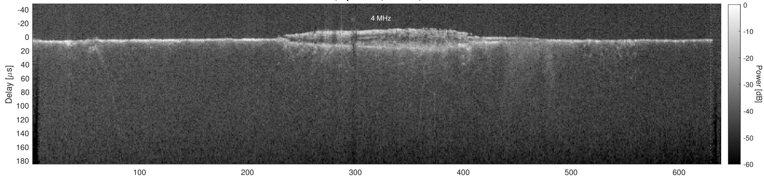
Orbit 18049, Cluttergram
