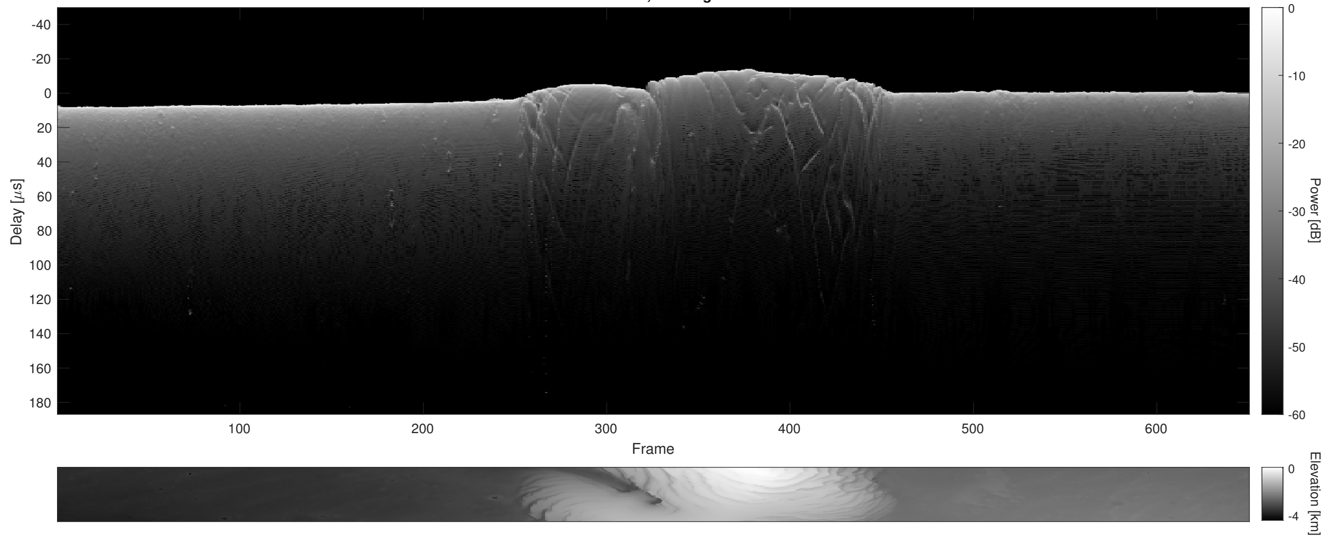
Orbit 18053, Cluttergram
