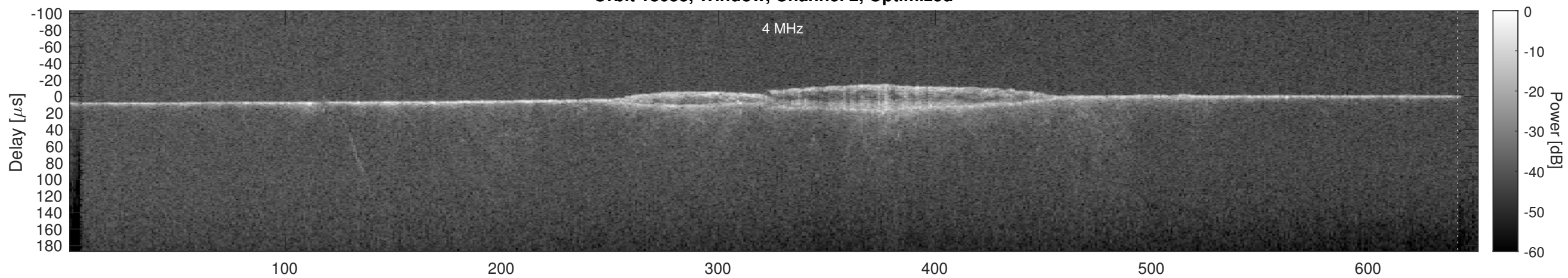
Orbit 18053, Cluttergram
