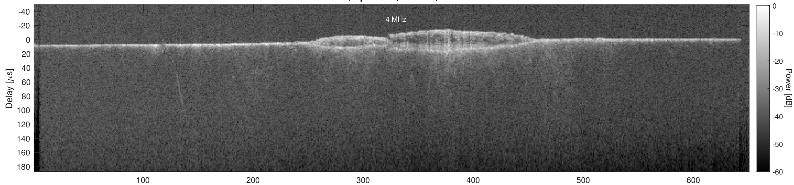
Orbit 18053, Cluttergram
