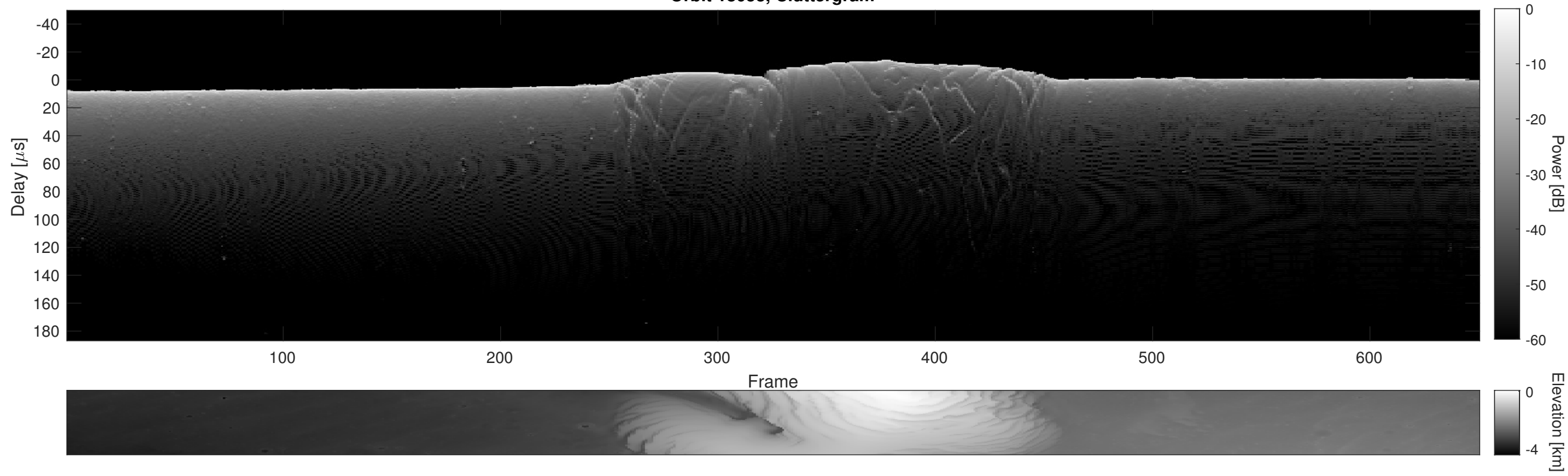
Orbit 18053, Cluttergram
