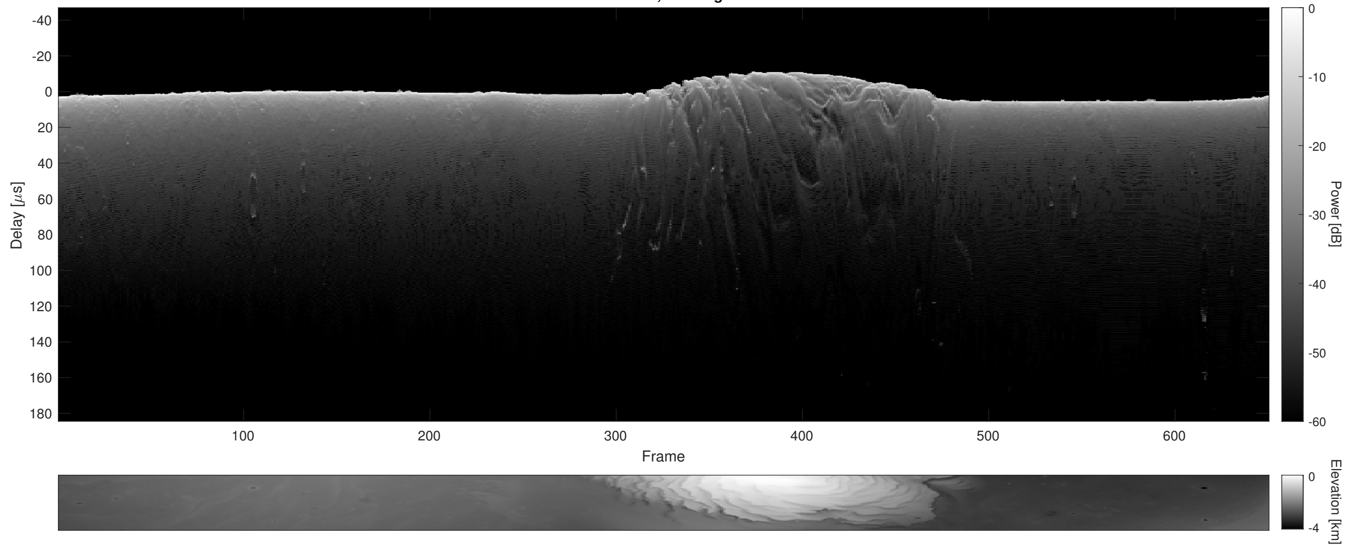
Orbit 18055, Cluttergram
