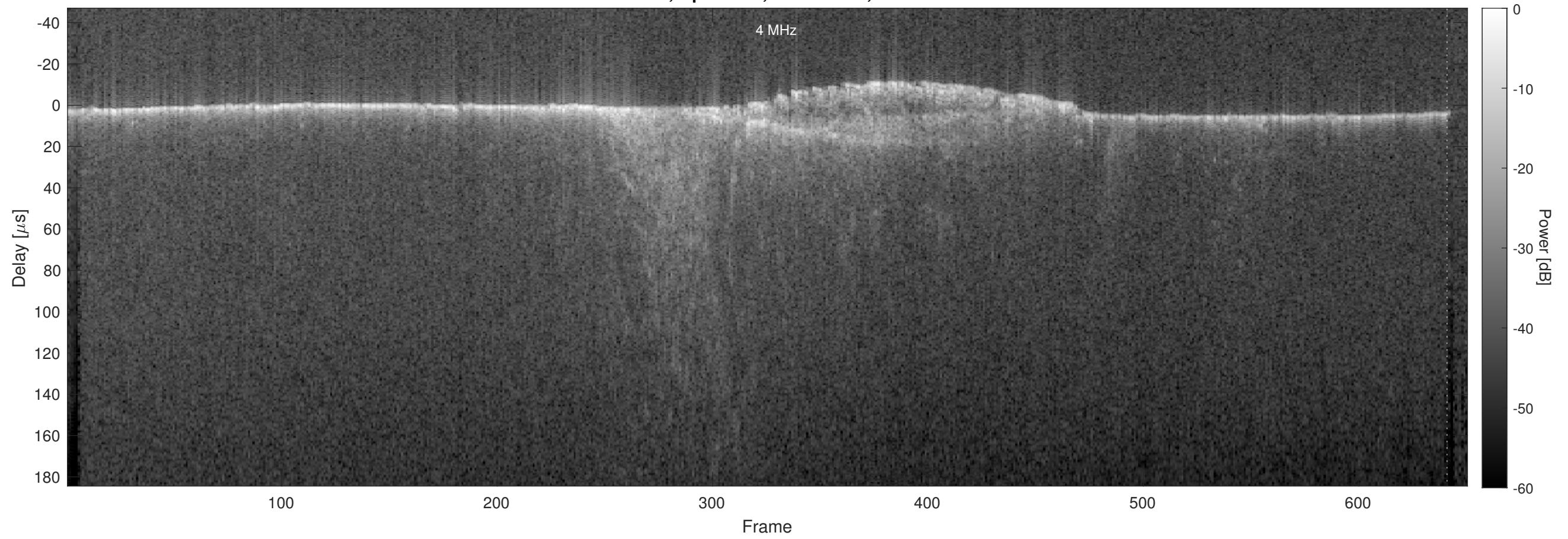
Orbit 18055, Optimized, No Window, Channel 2
