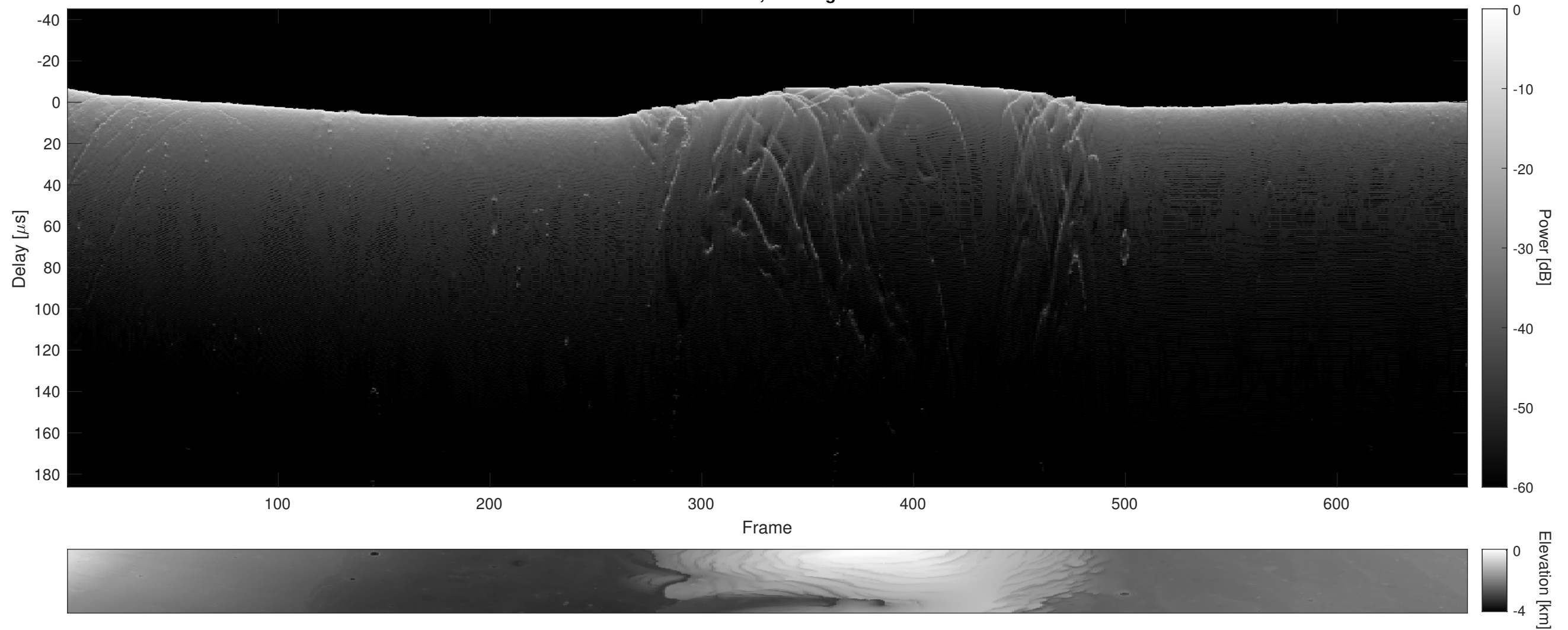
Orbit 18057, Cluttergram
