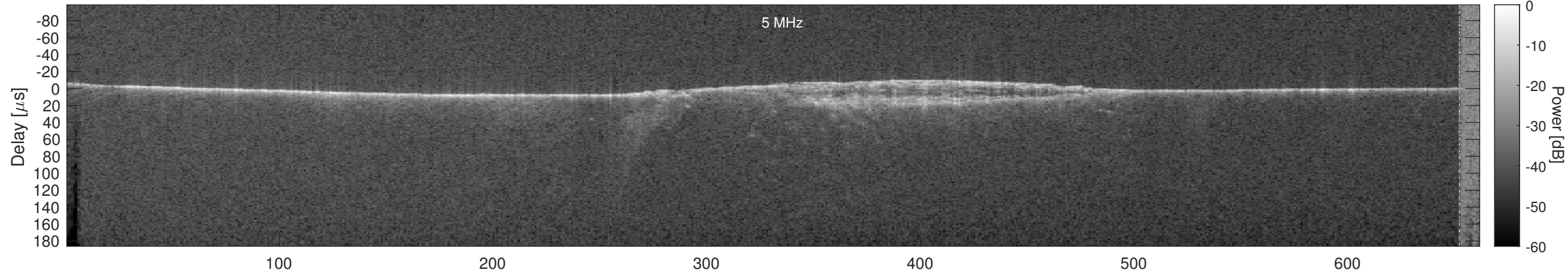
Orbit 18057, Cluttergram
