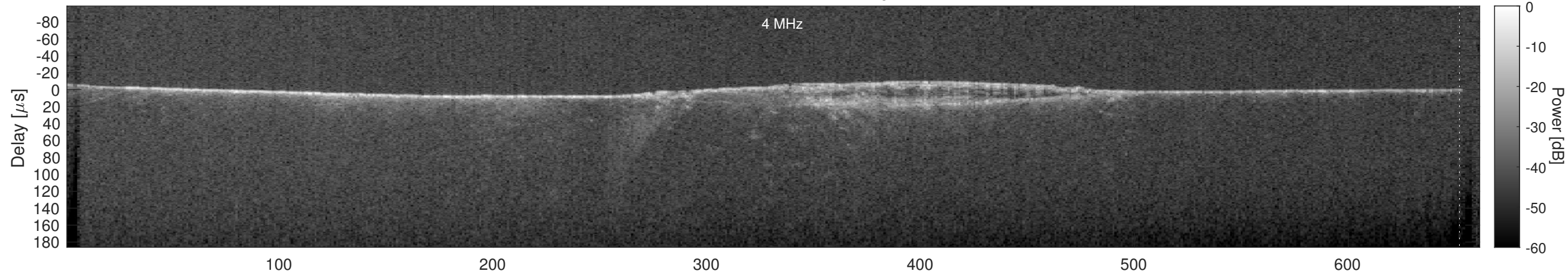
Orbit 18057, Cluttergram
