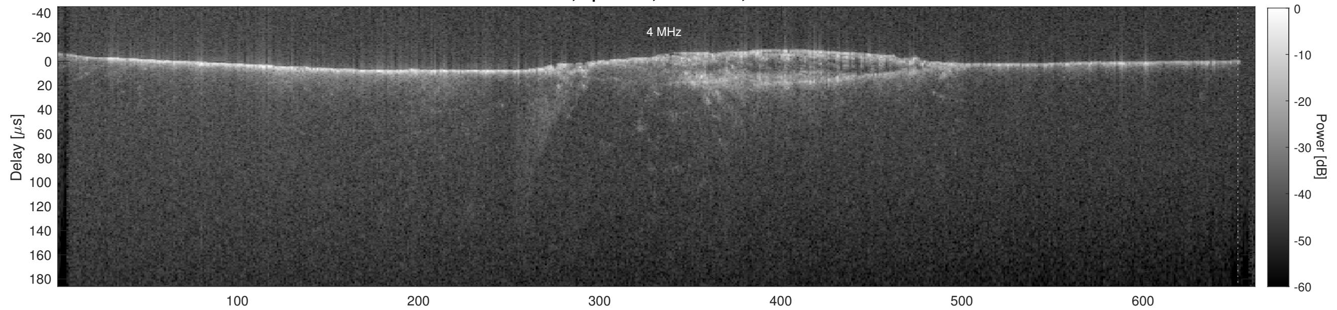
Orbit 18057, Cluttergram
