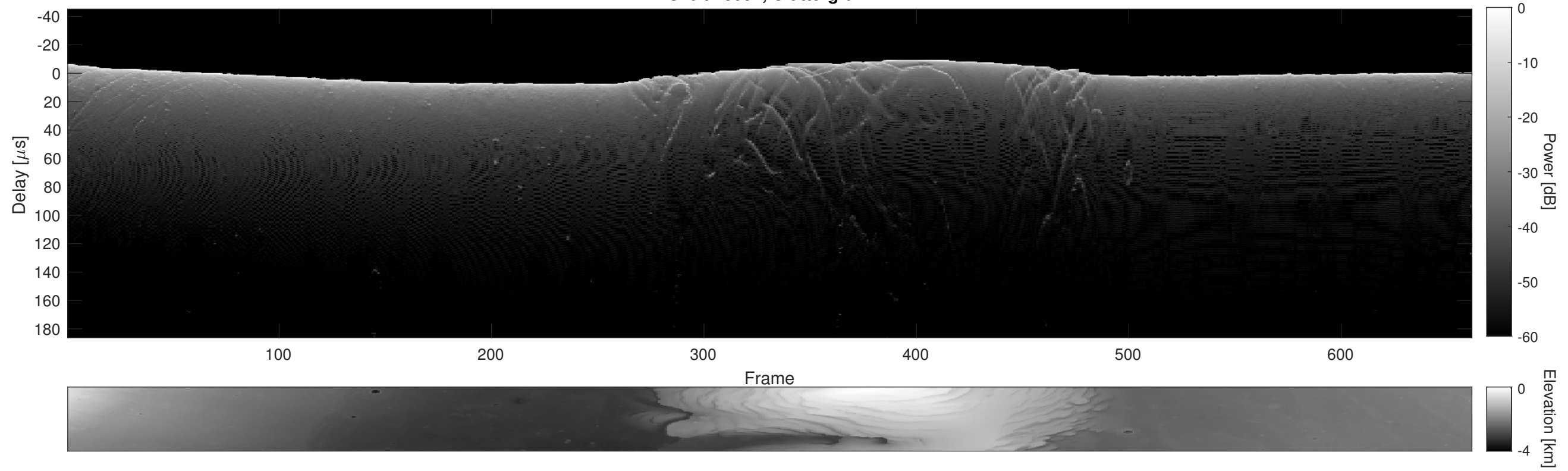
Orbit 18057, Cluttergram
