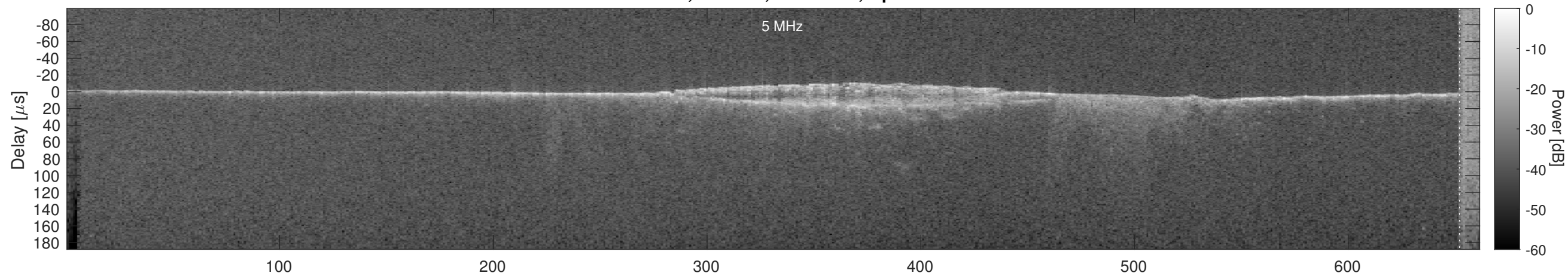
Orbit 18059, Cluttergram
