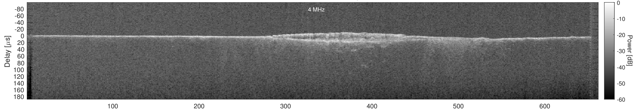
Orbit 18059, Cluttergram
