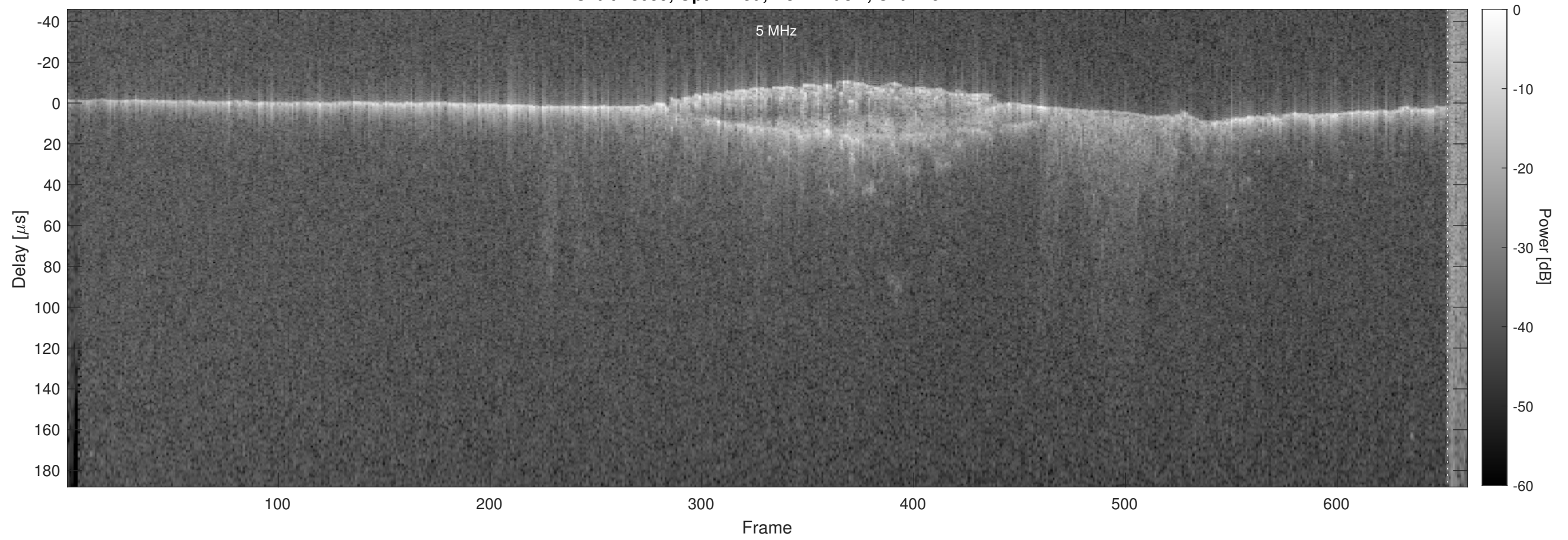
Orbit 18059, Optimized, No Window, Channel 2
