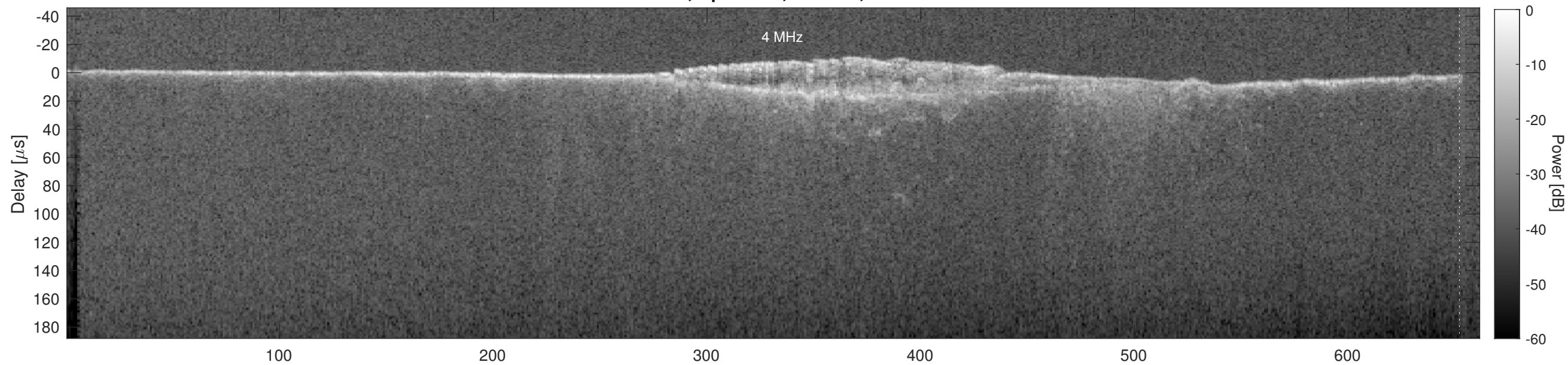
Orbit 18059, Cluttergram
