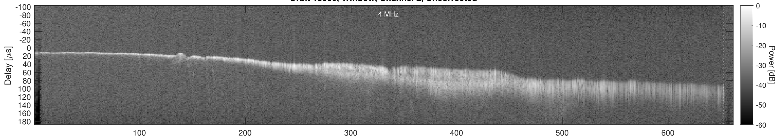
Orbit 18060, Window, Channel 2, Chapman
