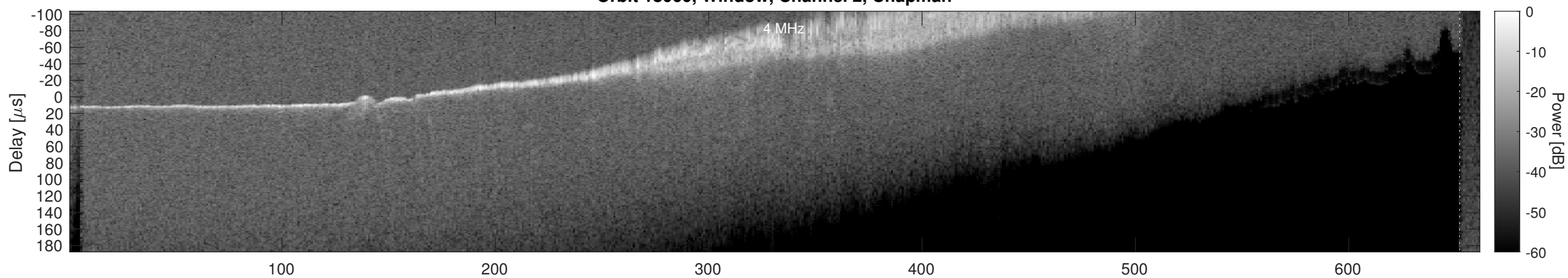
Orbit 18060, Window, Channel 2, Optimized
