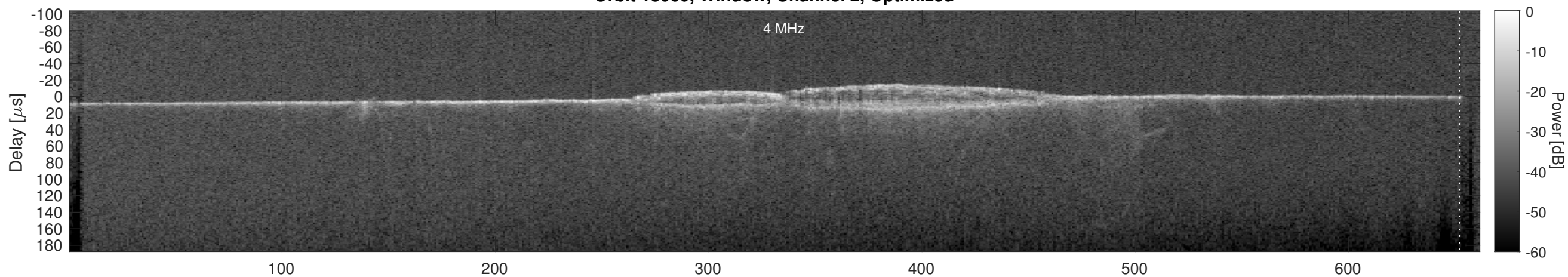
Orbit 18060, Cluttergram
