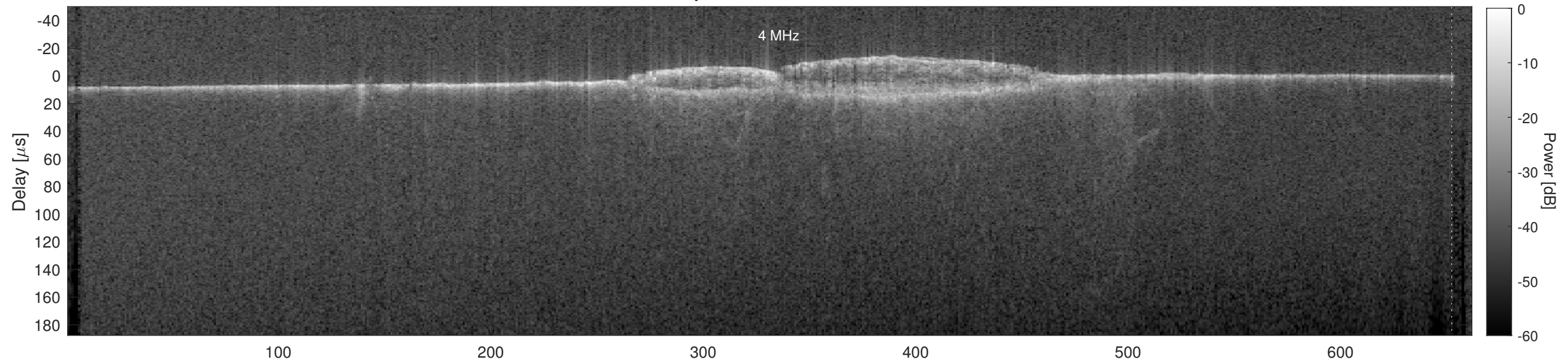
Orbit 18060, Cluttergram
