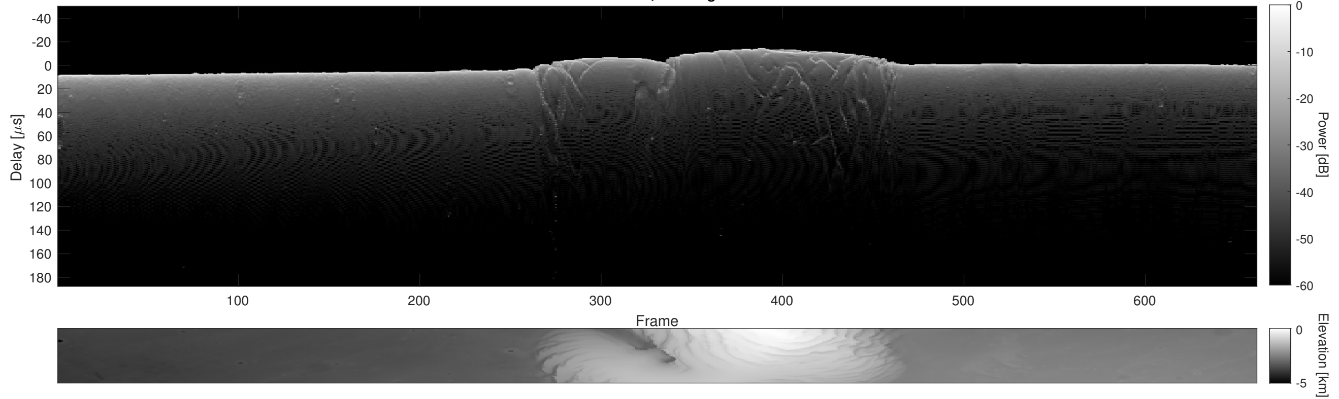
Orbit 18060, Cluttergram
