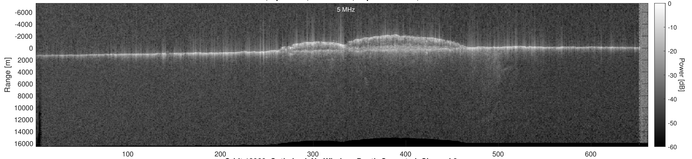
Orbit 18060, Optimized, No Window, Depth-Corrected, Channel 2
