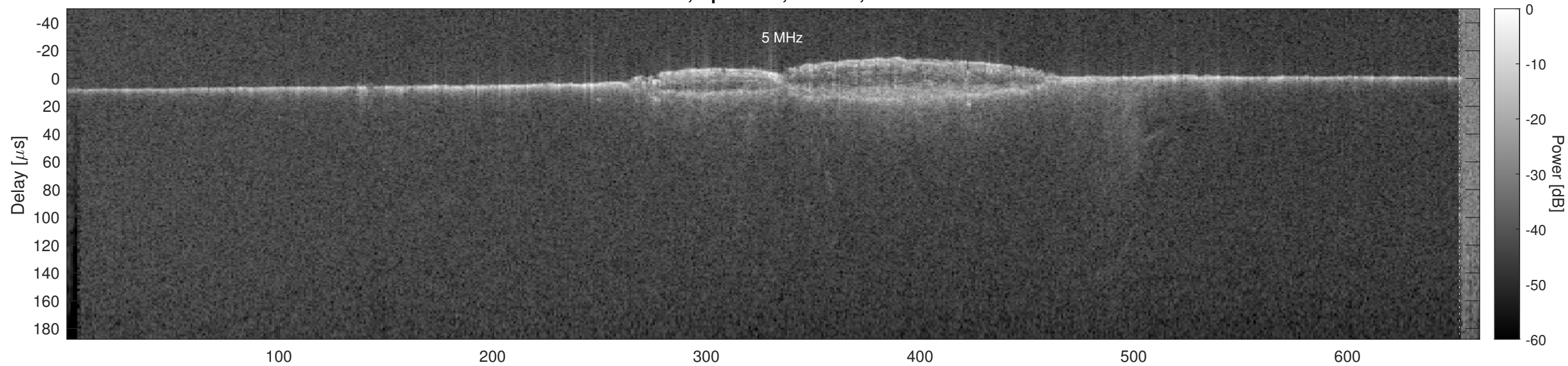
Orbit 18060, Optimized, Window, Channel 2
