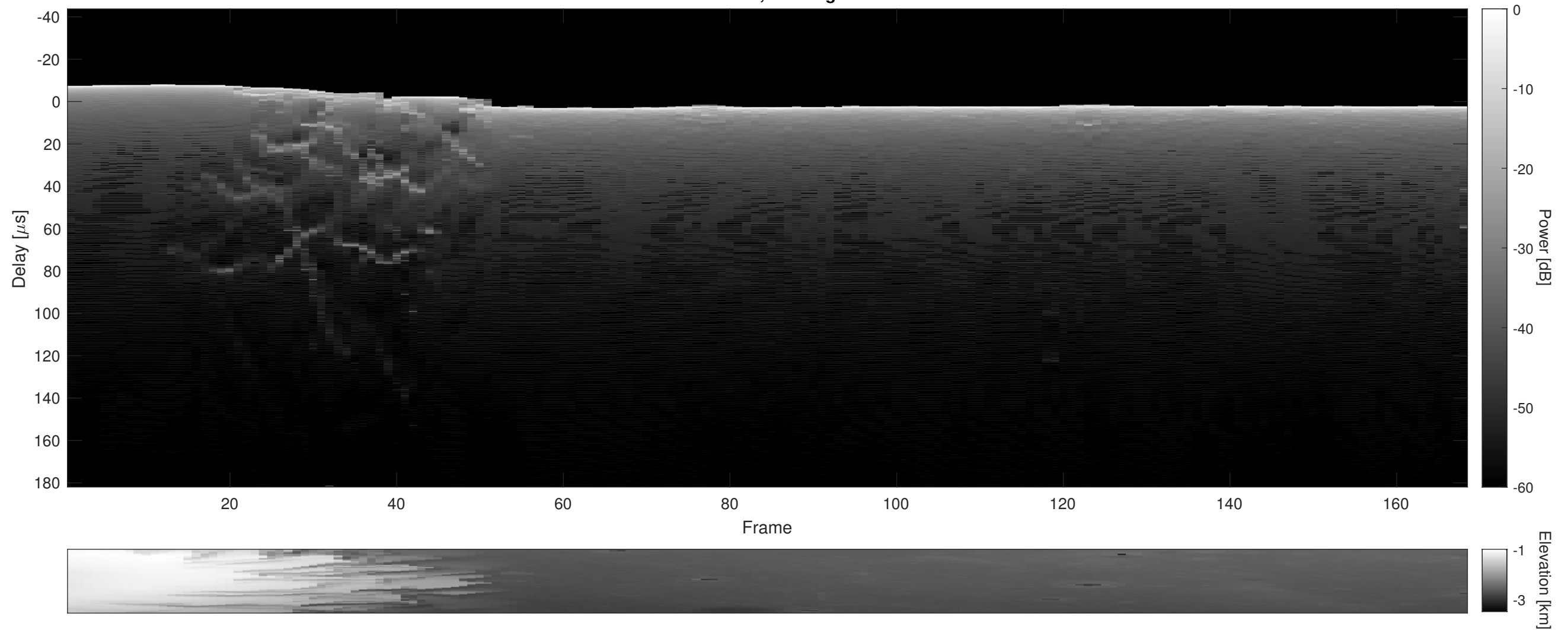
Orbit 18135, Cluttergram
