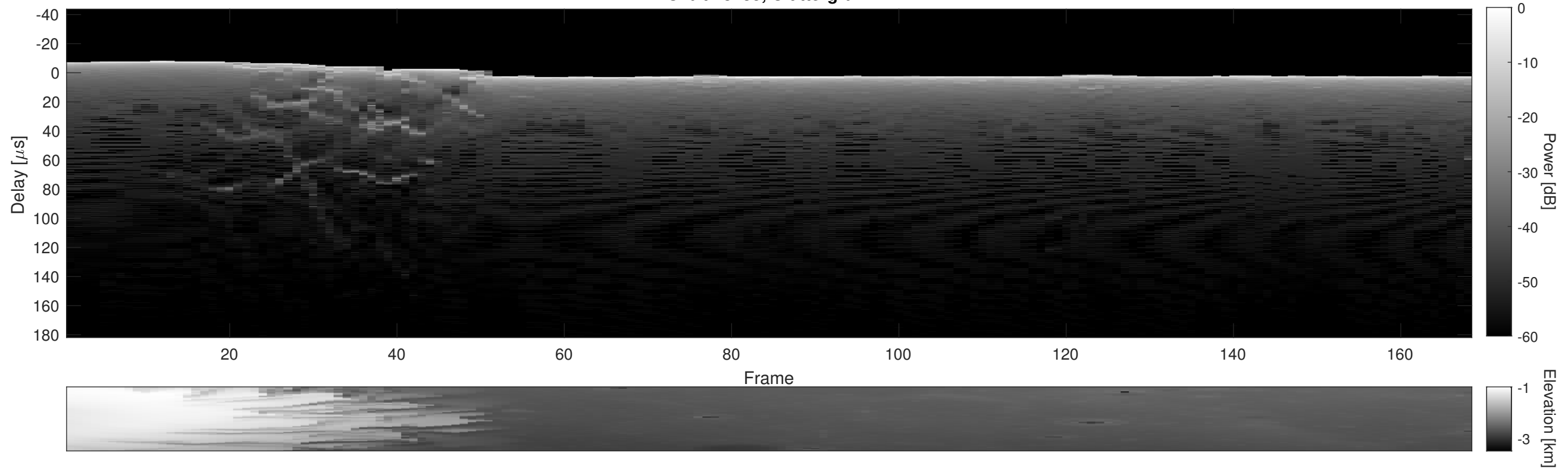
Orbit 18135, Cluttergram
