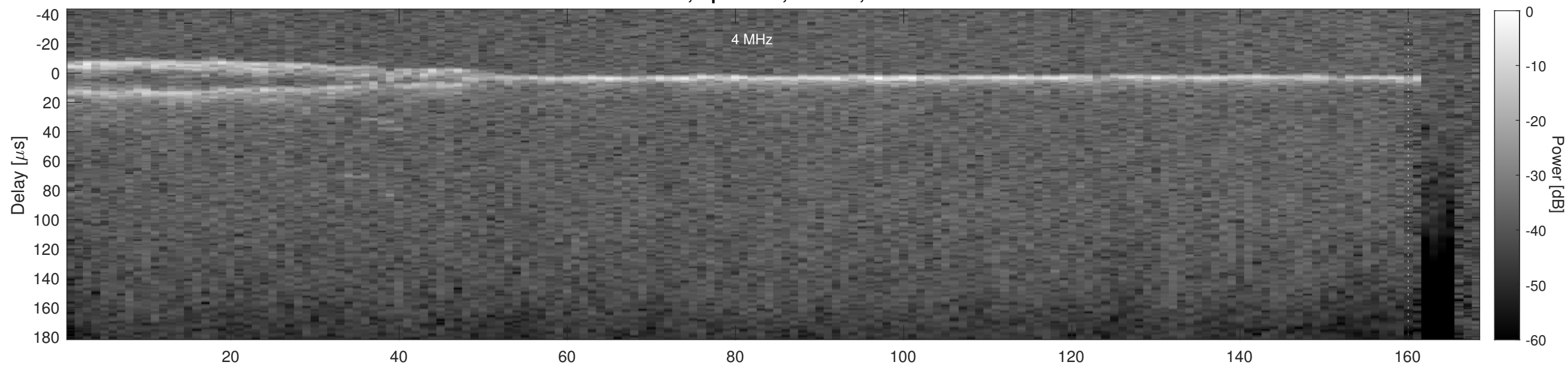
Orbit 18135, Cluttergram
