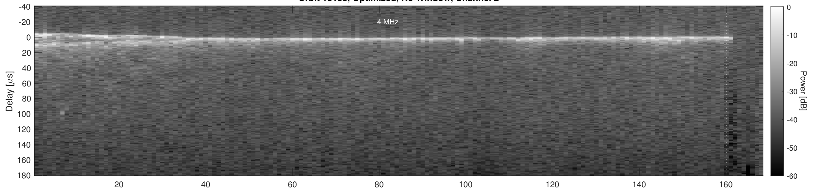
Orbit 18138, Cluttergram
