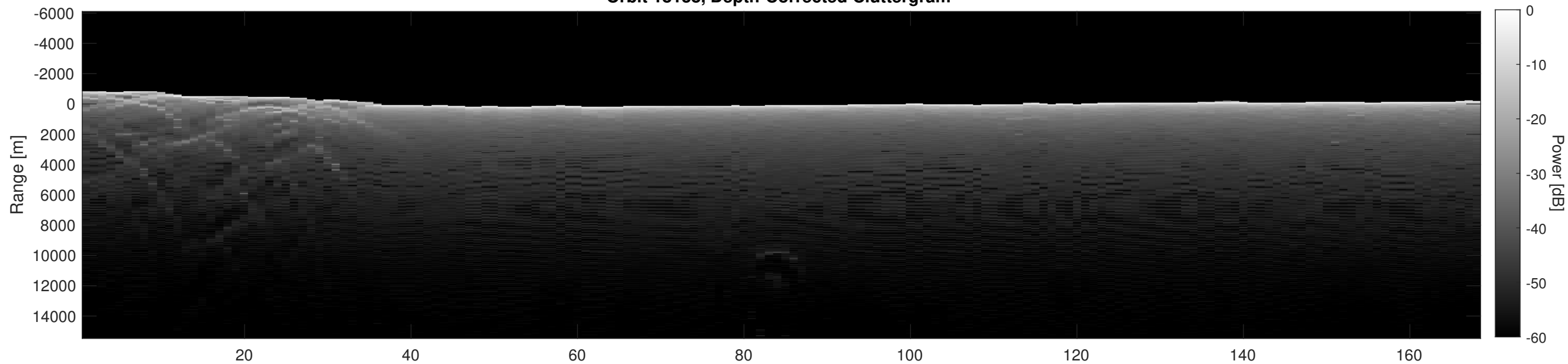
Orbit 18138, Depth-Corrected Cluttergram
