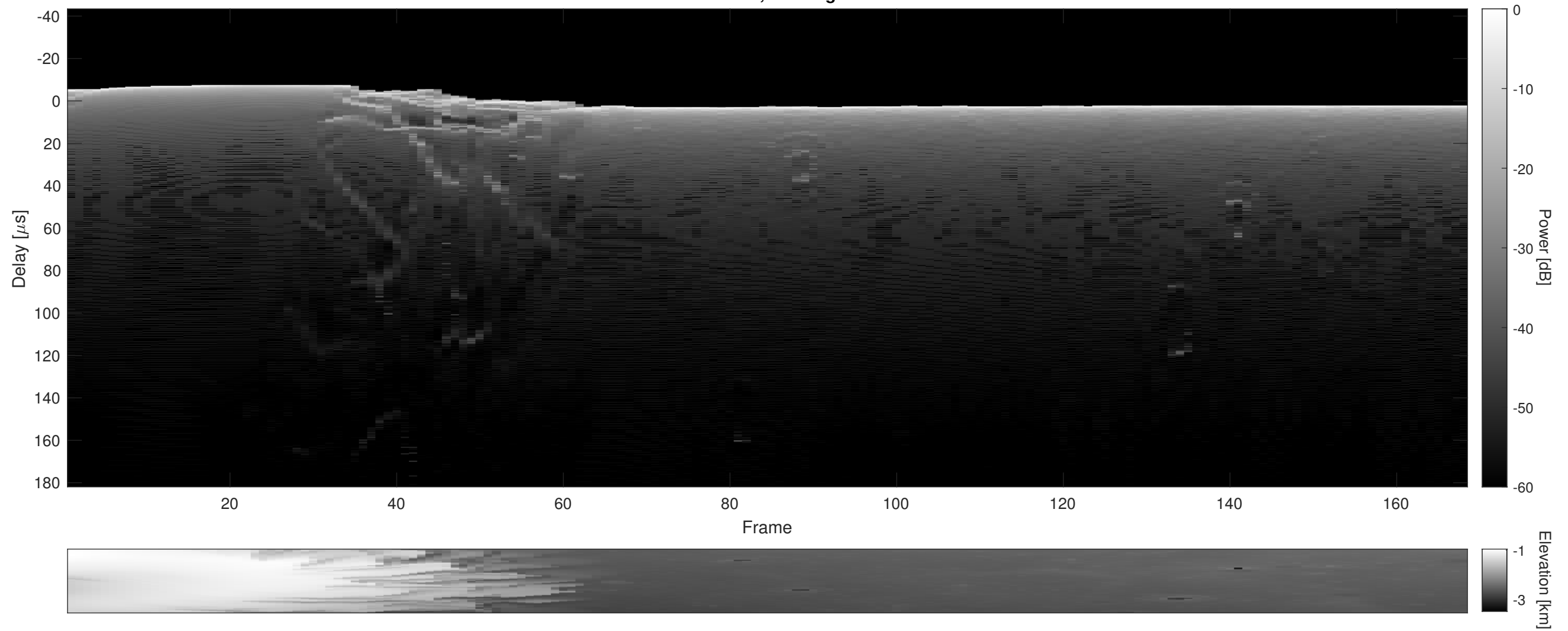
Orbit 18142, Cluttergram
