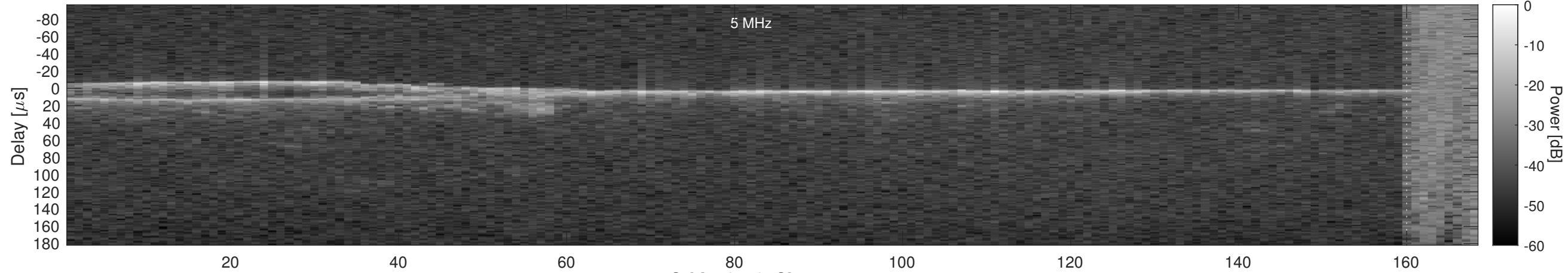
Orbit 18142, Cluttergram
