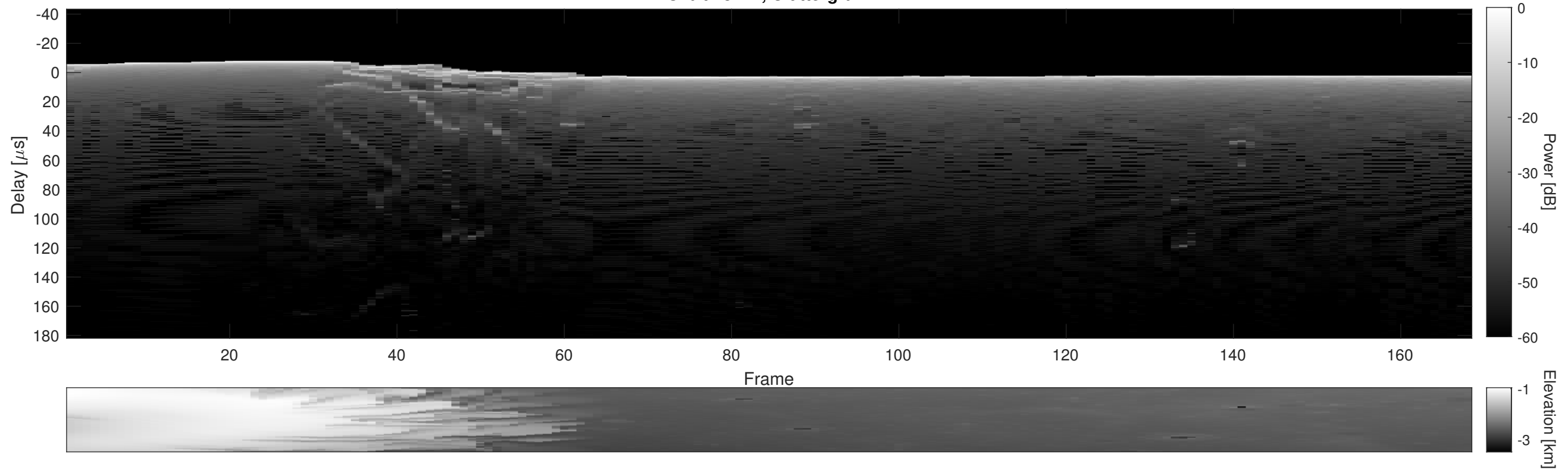
Orbit 18142, Cluttergram
