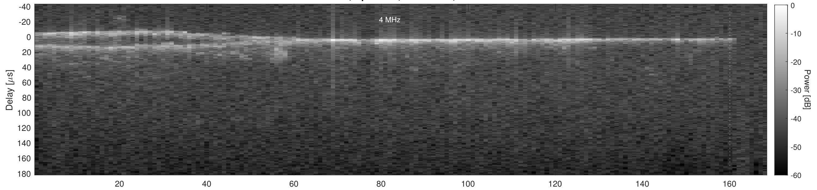
Orbit 18142, Cluttergram
