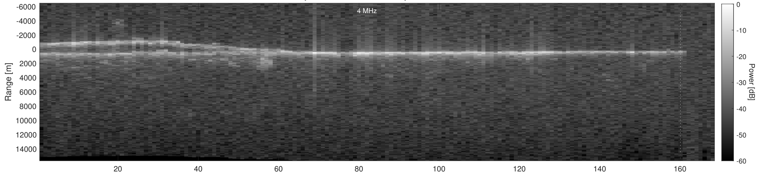
Orbit 18142, Depth-Corrected Cluttergram
