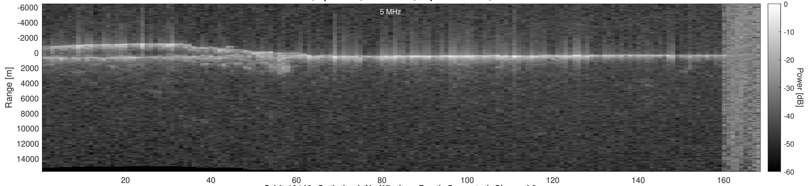
Orbit 18142, Optimized, No Window, Depth-Corrected, Channel 2
