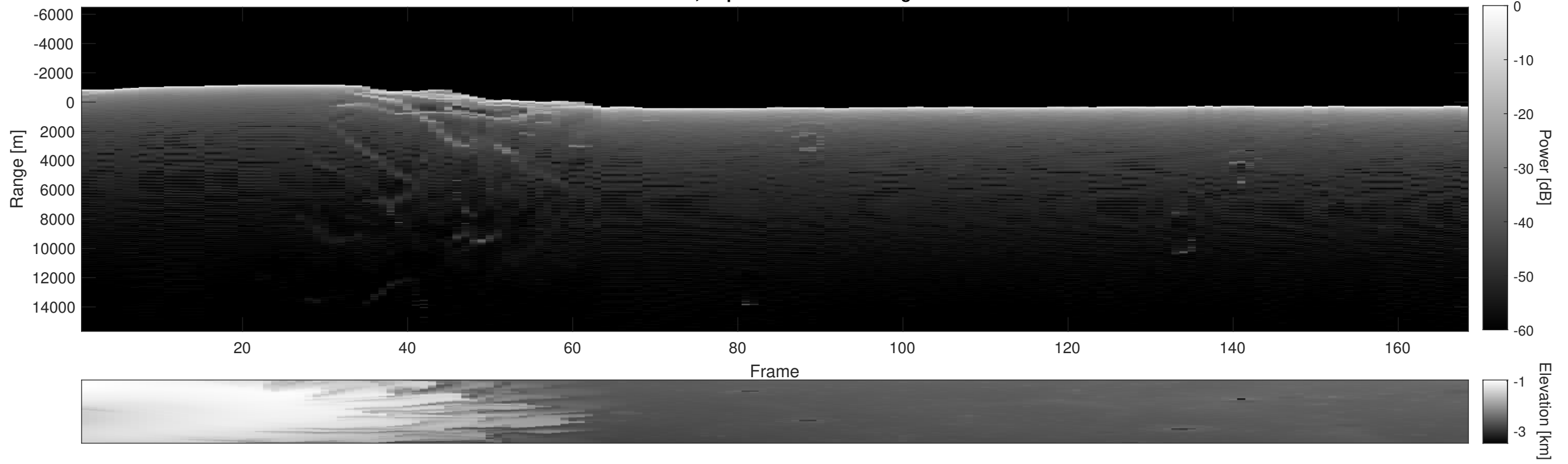
Orbit 18142, Depth-Corrected Cluttergram
