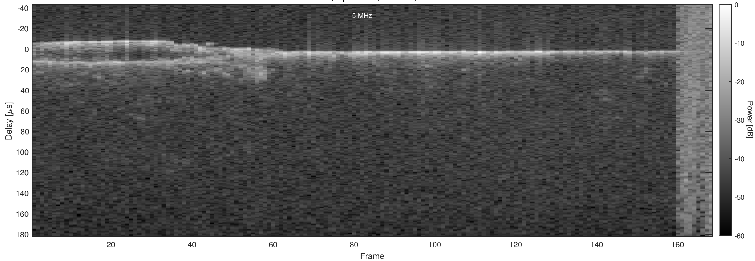
Orbit 18142, Optimized, Window, Channel 2
