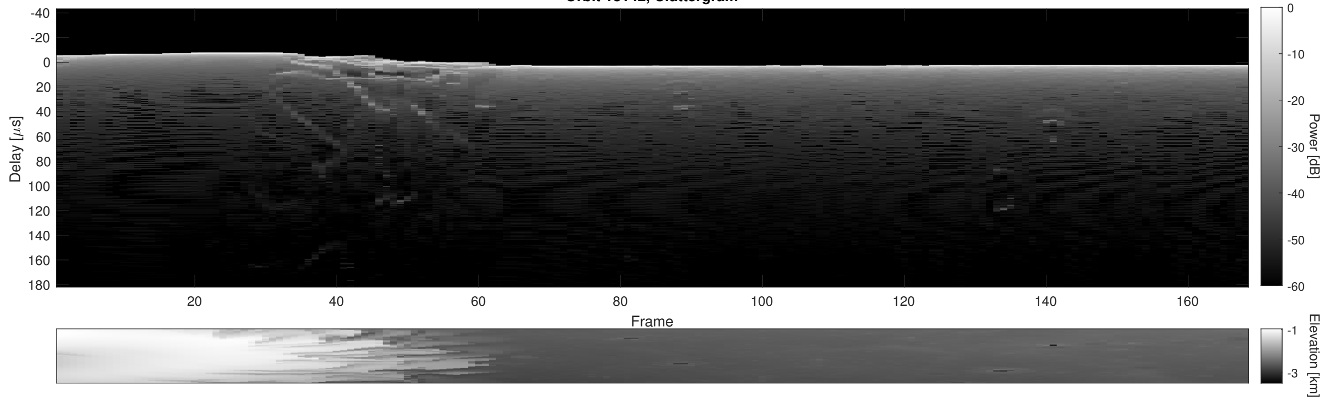
Orbit 18142, Cluttergram
