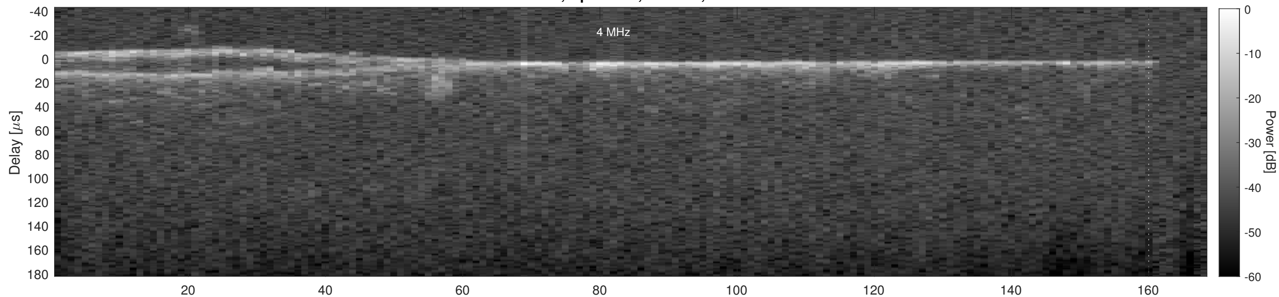
Orbit 18142, Cluttergram
