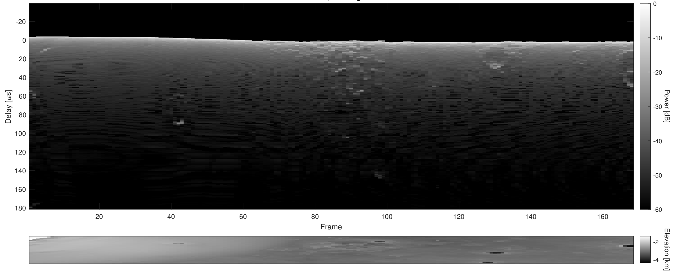
Orbit 18144, Cluttergram
