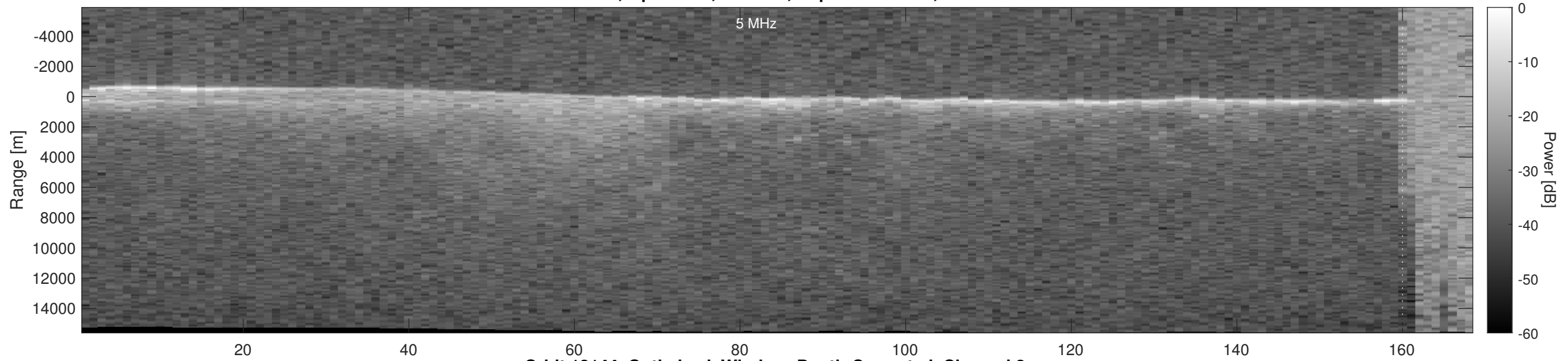
Orbit 18144, Optimized, Window, Depth-Corrected, Channel 2
