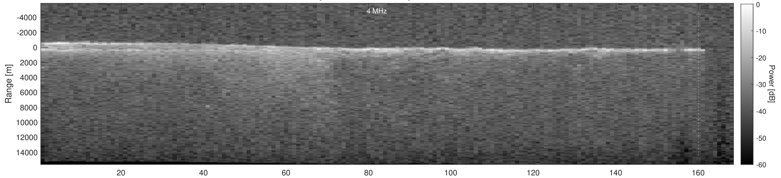
Orbit 18144, Depth-Corrected Cluttergram
