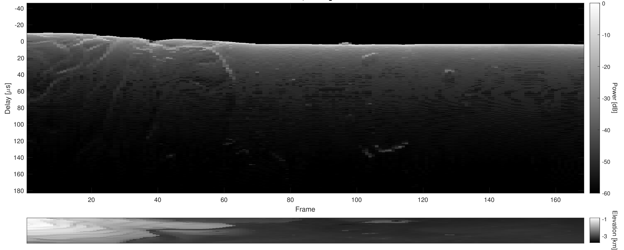
Orbit 18150, Cluttergram
