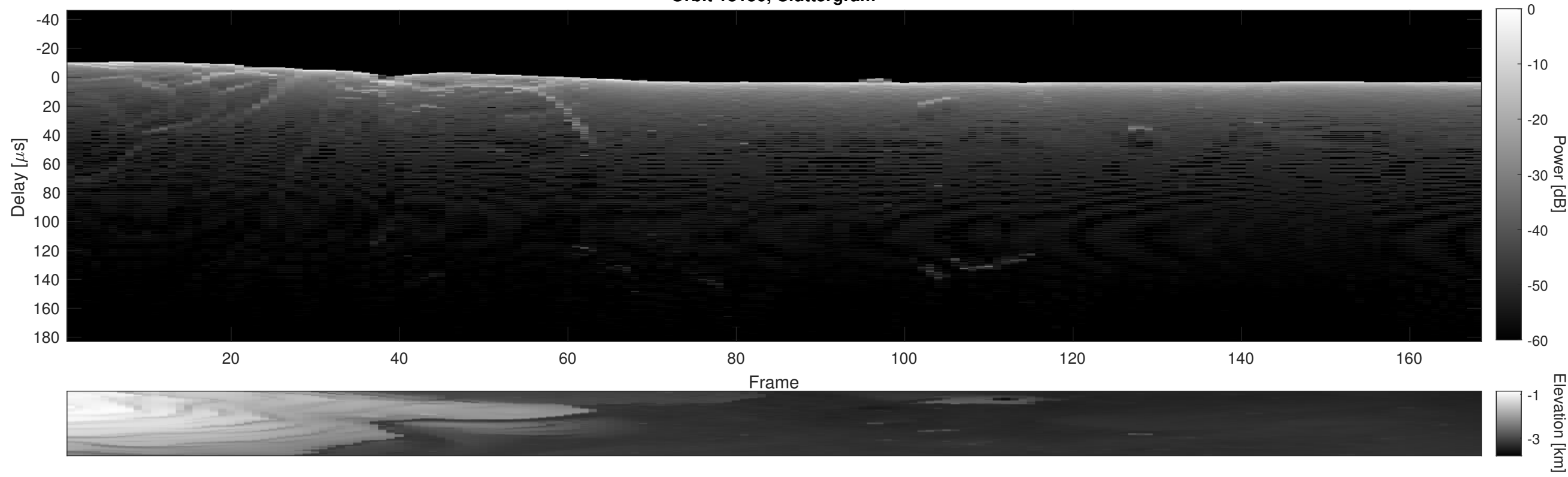
Orbit 18150, Cluttergram
