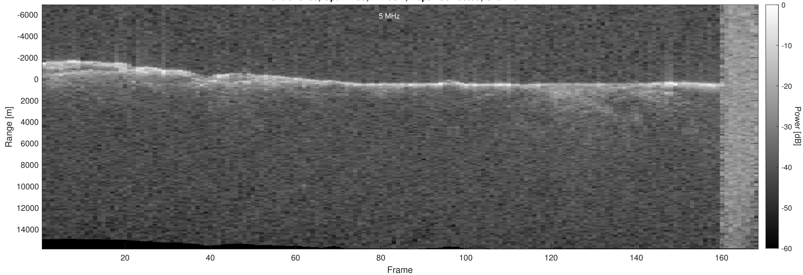
Orbit 18150, Optimized, Window, Depth-Corrected, Channel 2
