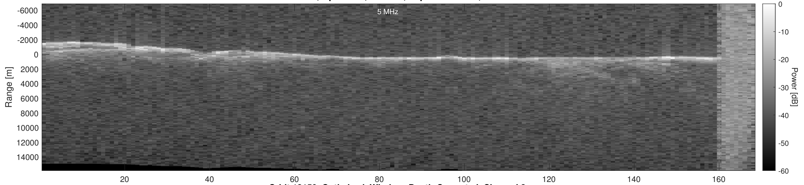
Orbit 18150, Optimized, Window, Depth-Corrected, Channel 2
