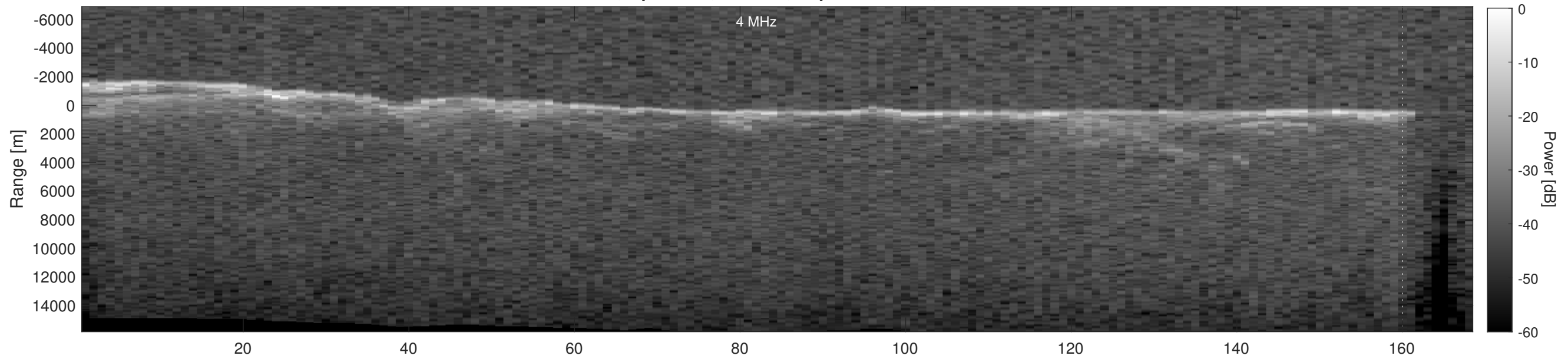
Orbit 18150, Depth-Corrected Cluttergram
