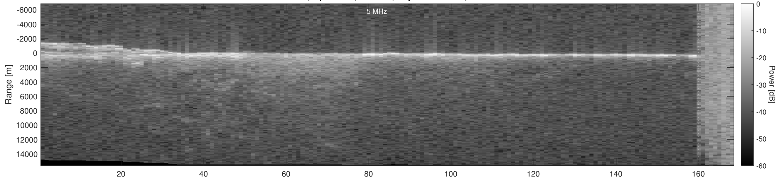
Orbit 18155, Optimized, Window, Depth-Corrected, Channel 2
