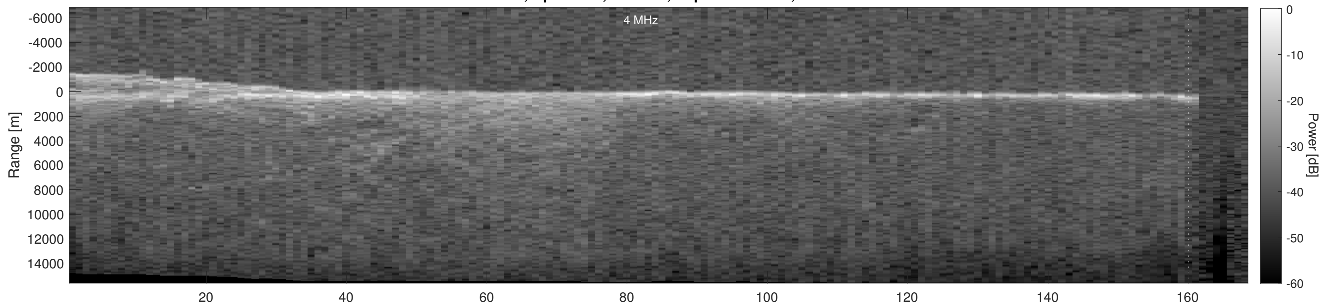
Orbit 18155, Depth-Corrected Cluttergram
