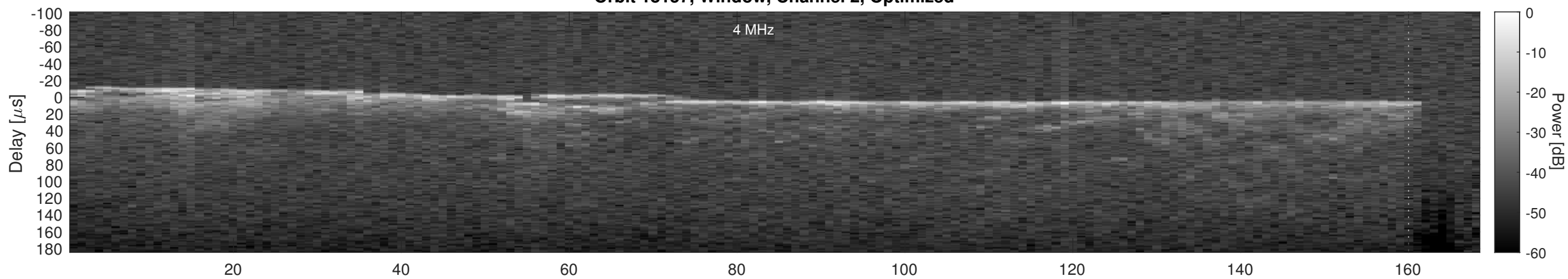
Orbit 18157, Cluttergram
