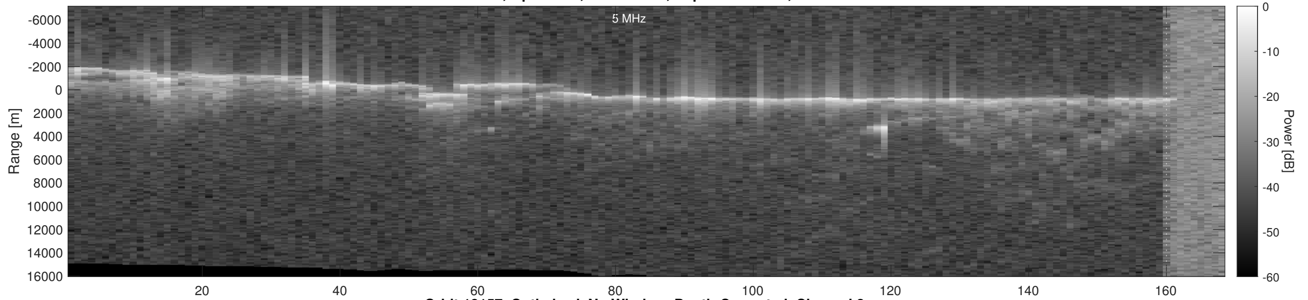
Orbit 18157, Optimized, No Window, Depth-Corrected, Channel 2
