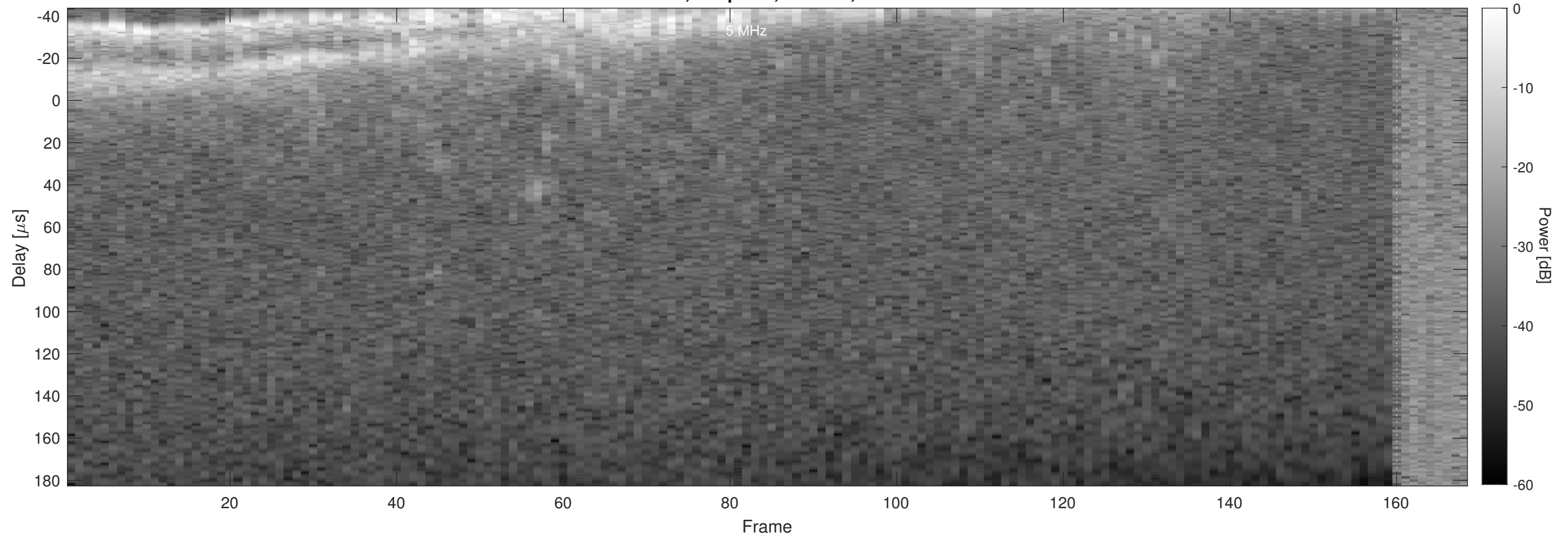
Orbit 18159, Chapman, Window, Channel 2
