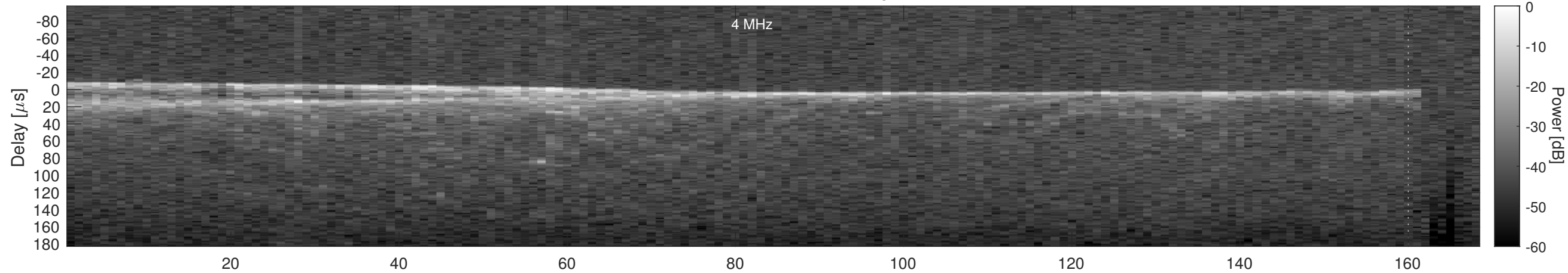
Orbit 18159, Cluttergram
