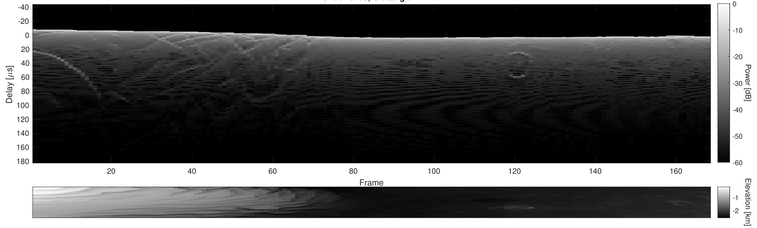
Orbit 18159, Cluttergram
