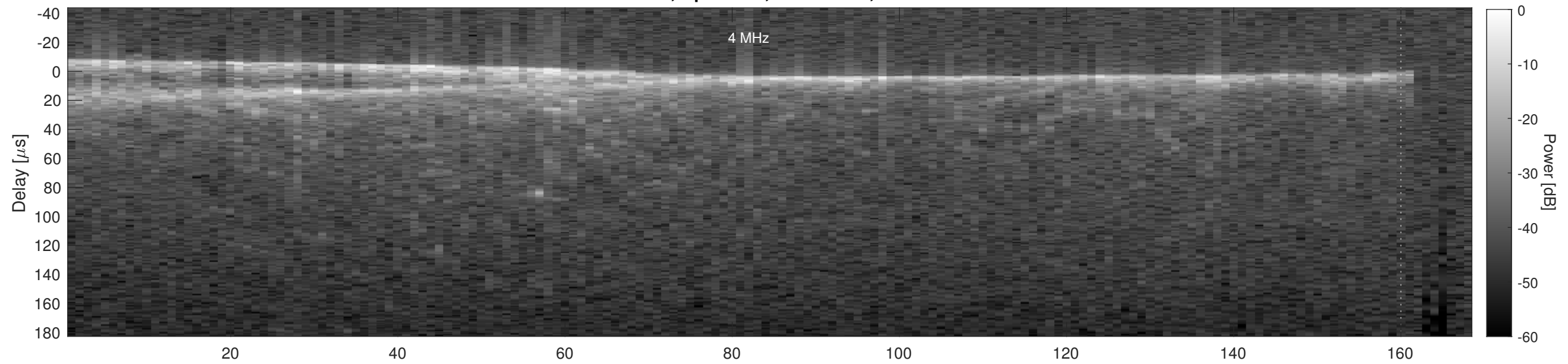
Orbit 18159, Cluttergram
